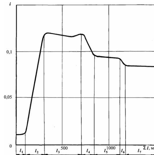
Fig. 4. Dependence of the slope longitudinal profile i on the length l Pershotravnevyi quarry road in the PJSC "Northern GZK" low horizons
