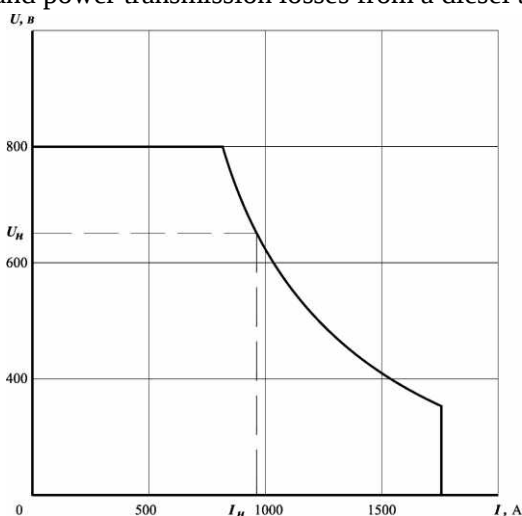
Fig. 1. External characteristic of the generator ( N_e = I_e \cdot U_e = \text{const} ) of the BelAZ-7549 dumper
